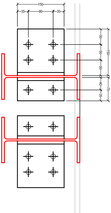
PLAN ON CONNECTION DETAIL
