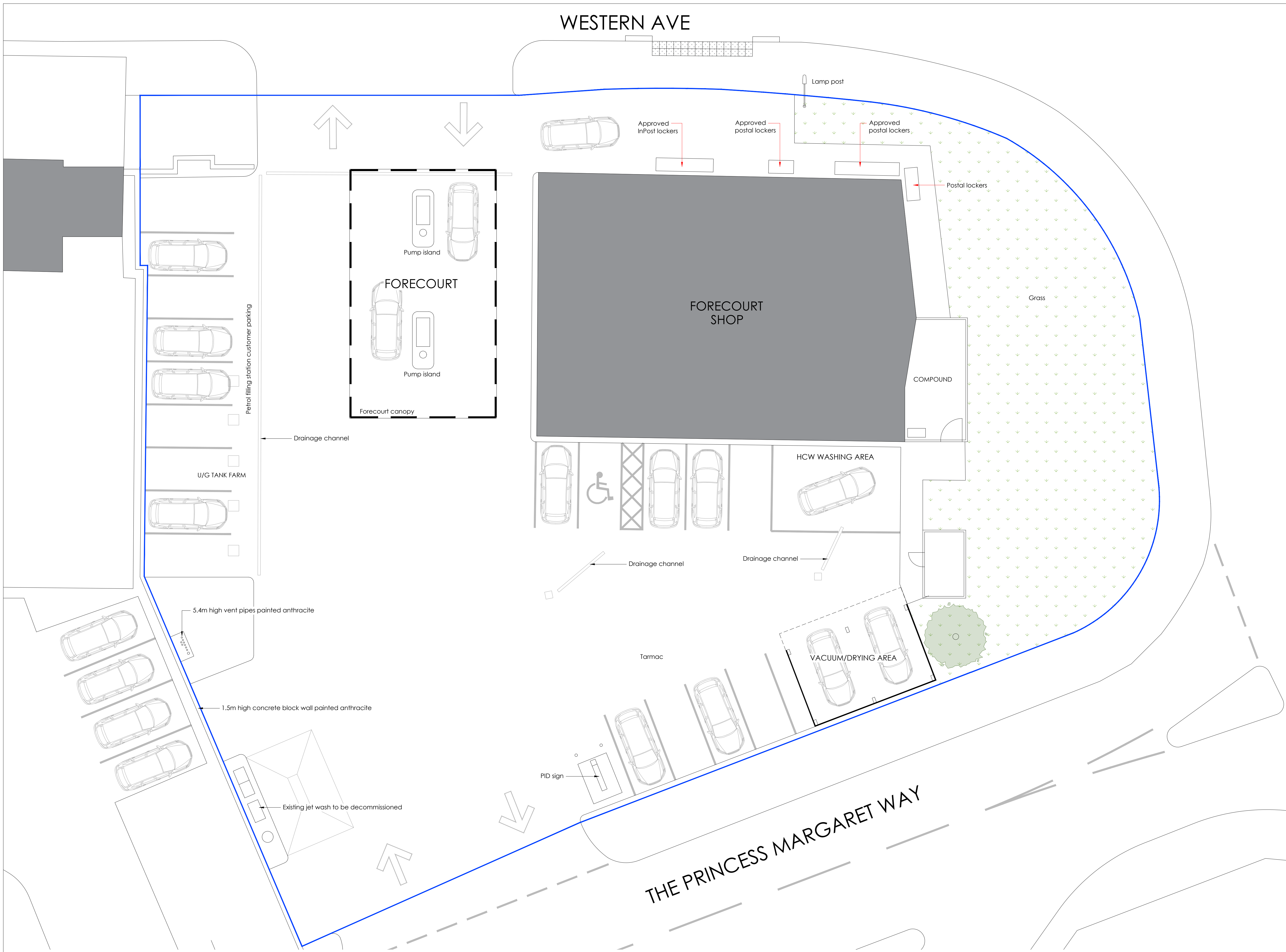
AS EXISTING SITE LAYOUT
