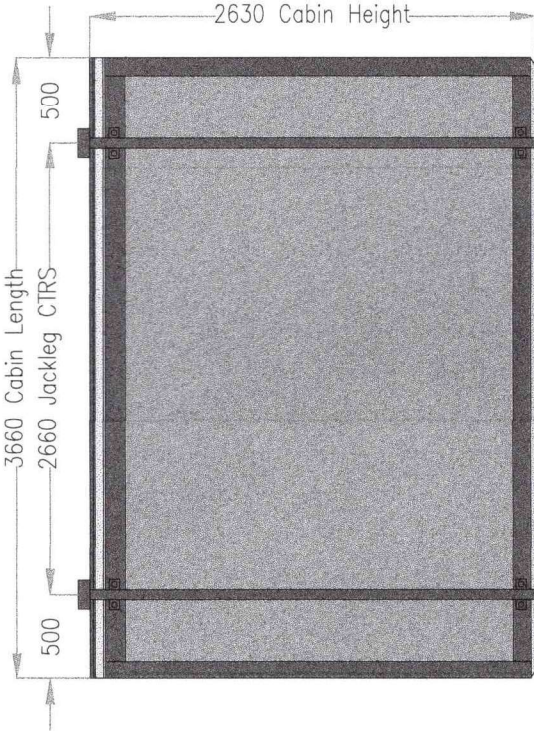
SIDE ELEVATION "B"
