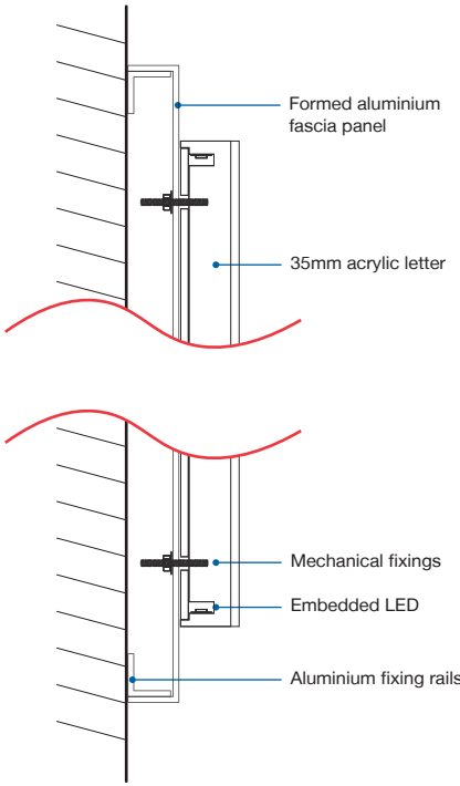
Section through - 1:5
