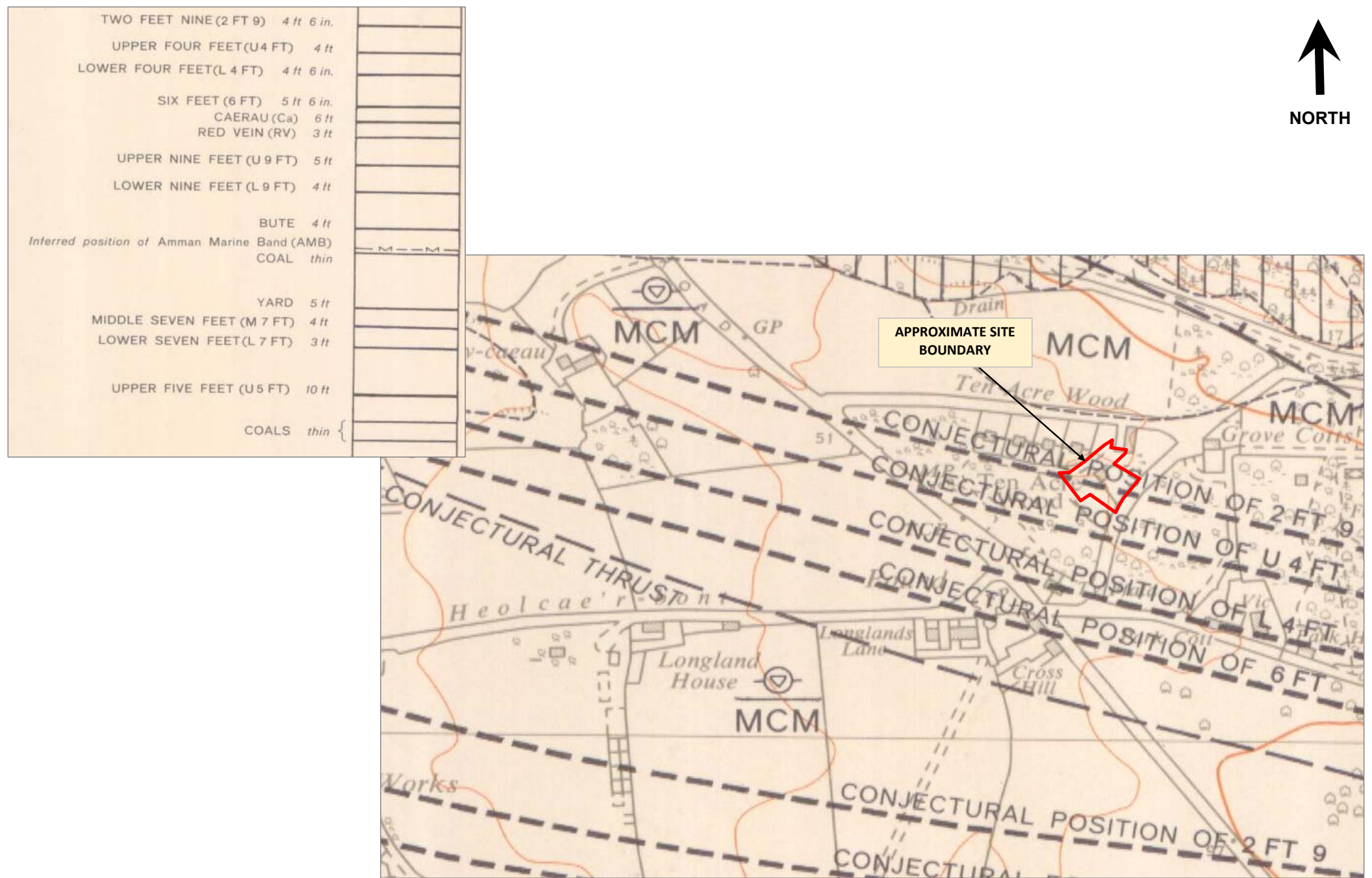
FIGURE 3: GEOLOGY MAP EXTRACT
