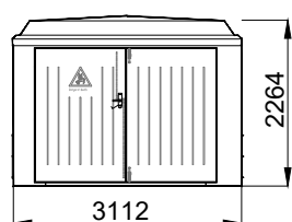
FRONT ELEVATION
