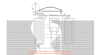
SIDE ELEVATION
