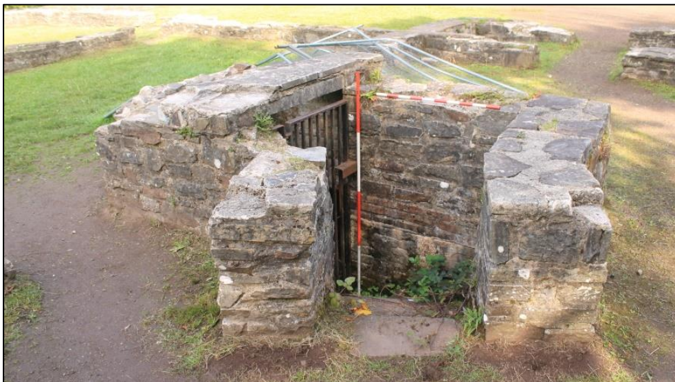
Photo 34: View northwest of Entrance 3 at surface level. 2m scale.
