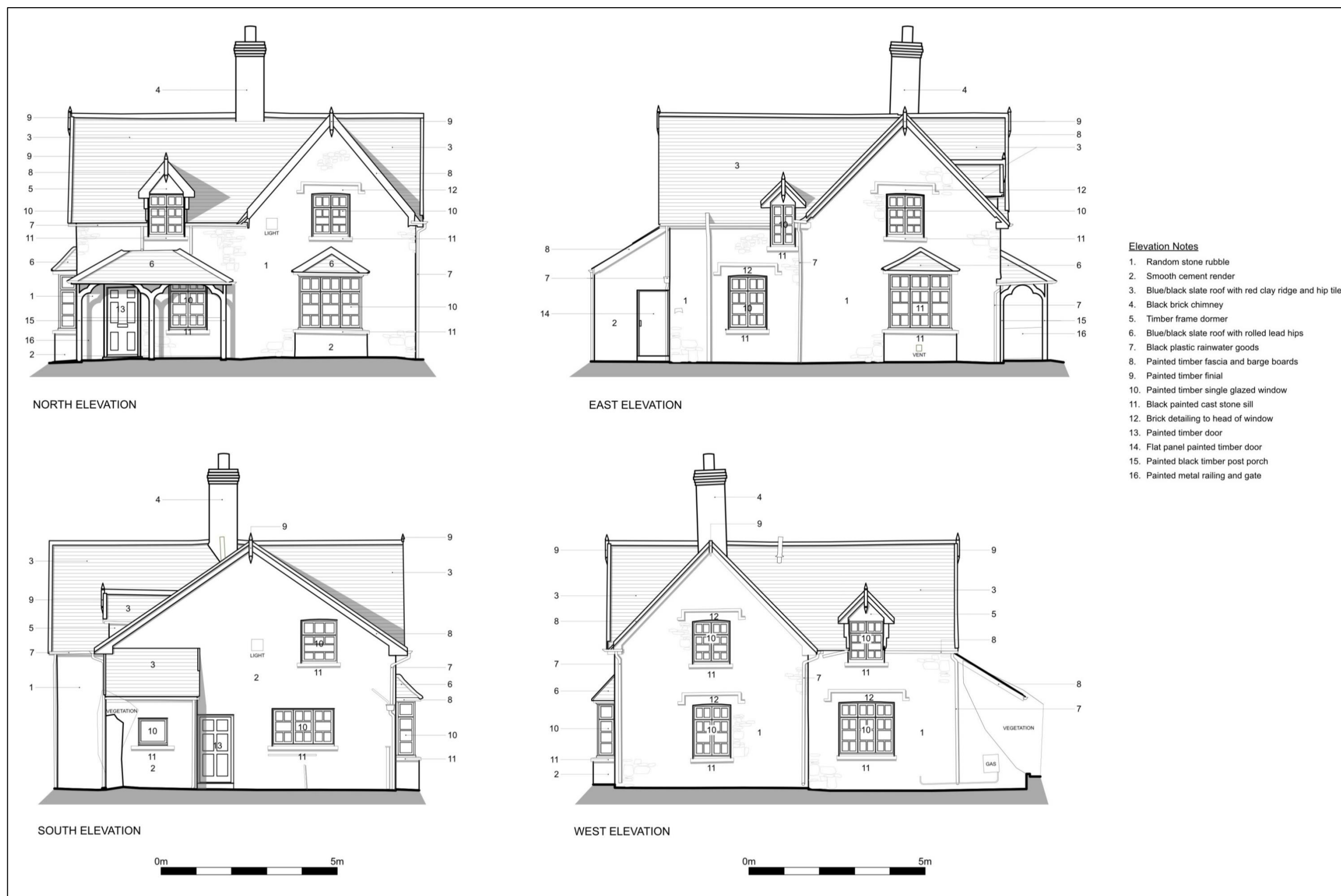
Figure 18: Elevations of Pond Cottage. Based on drawings produced by Hiraeth for Andrew Scott Ltd (drawing 03040/S0/P3) with adaptations and annotations by DAT-AS.
