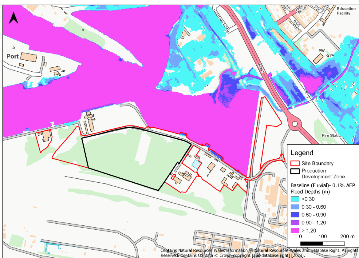
Figure 1-5 0.1% AEP plus climate change fluvial event
