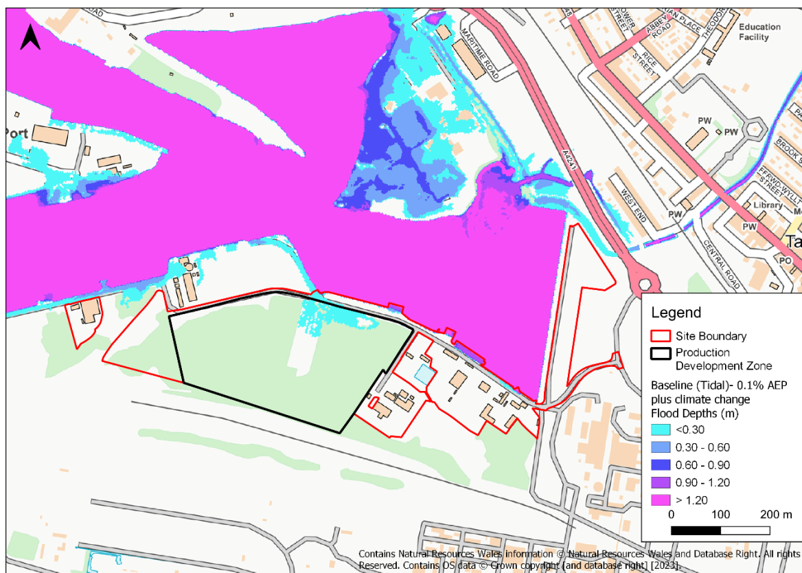
Figure 1-6 0.1% AEP plus climate change tidal event
