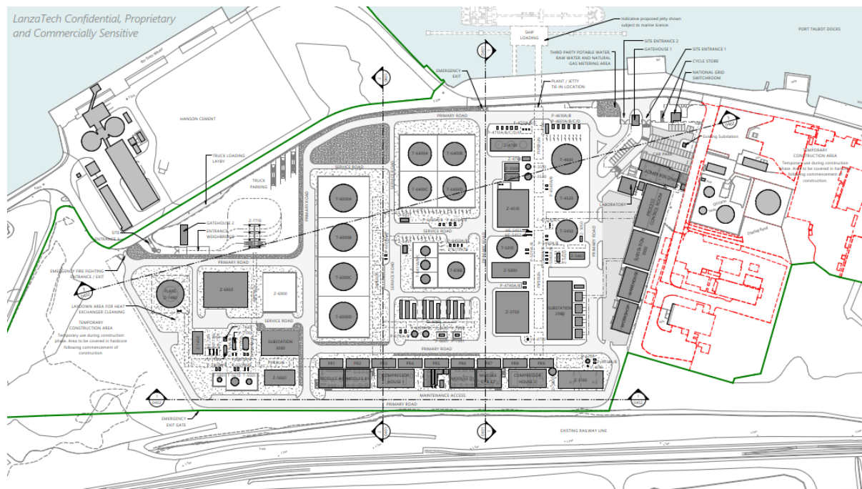
Figure 5-2 Project Dragon Proposed Site Arrangements
