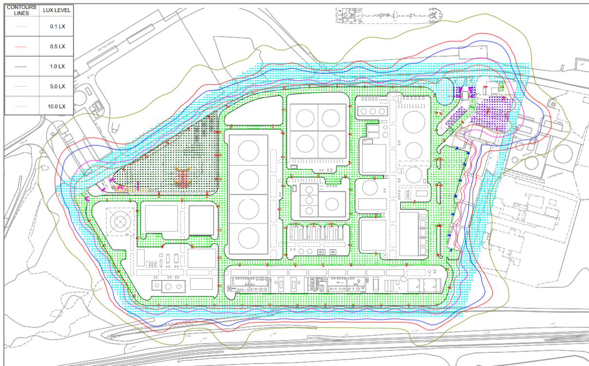
Figure 8-1 Exterior Lighting Isolux Plot
