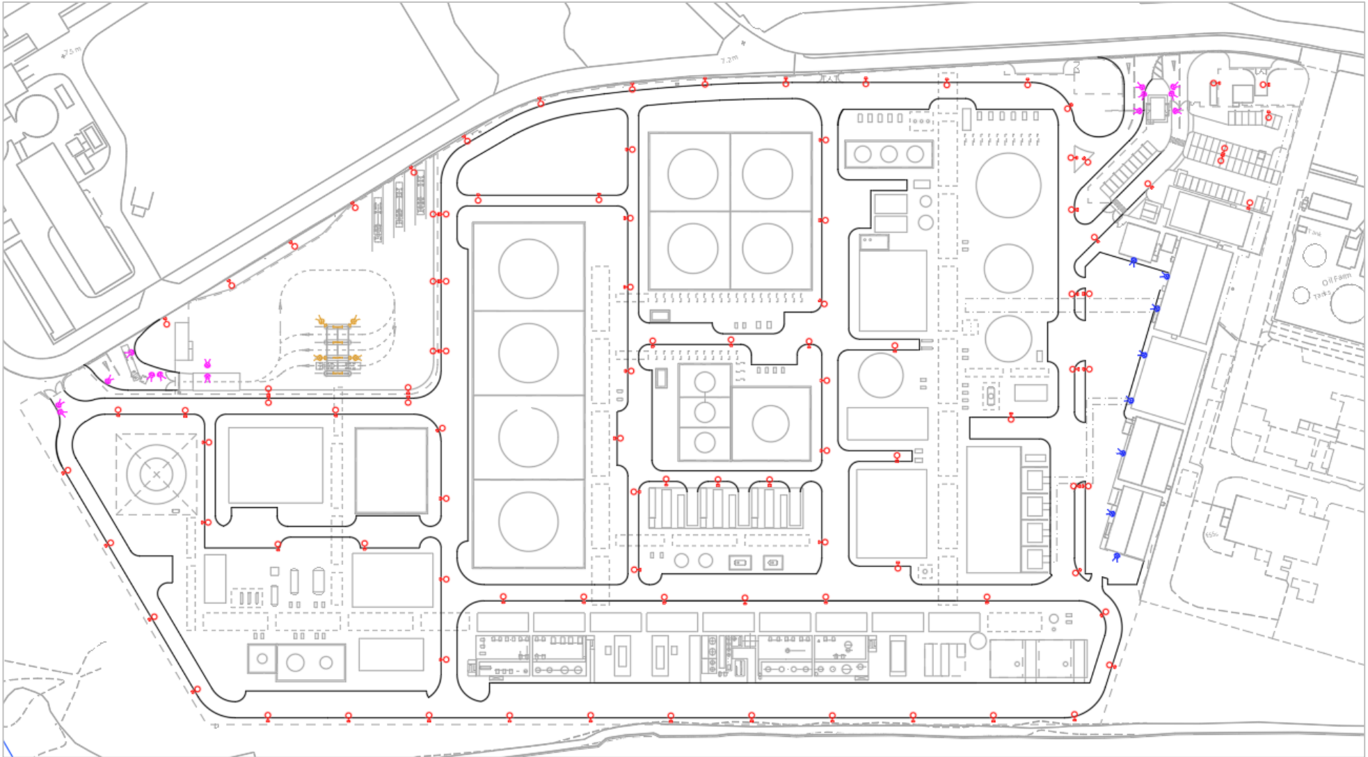
Figure 7-1 Proposed Lighting Layout – Ground Areas
