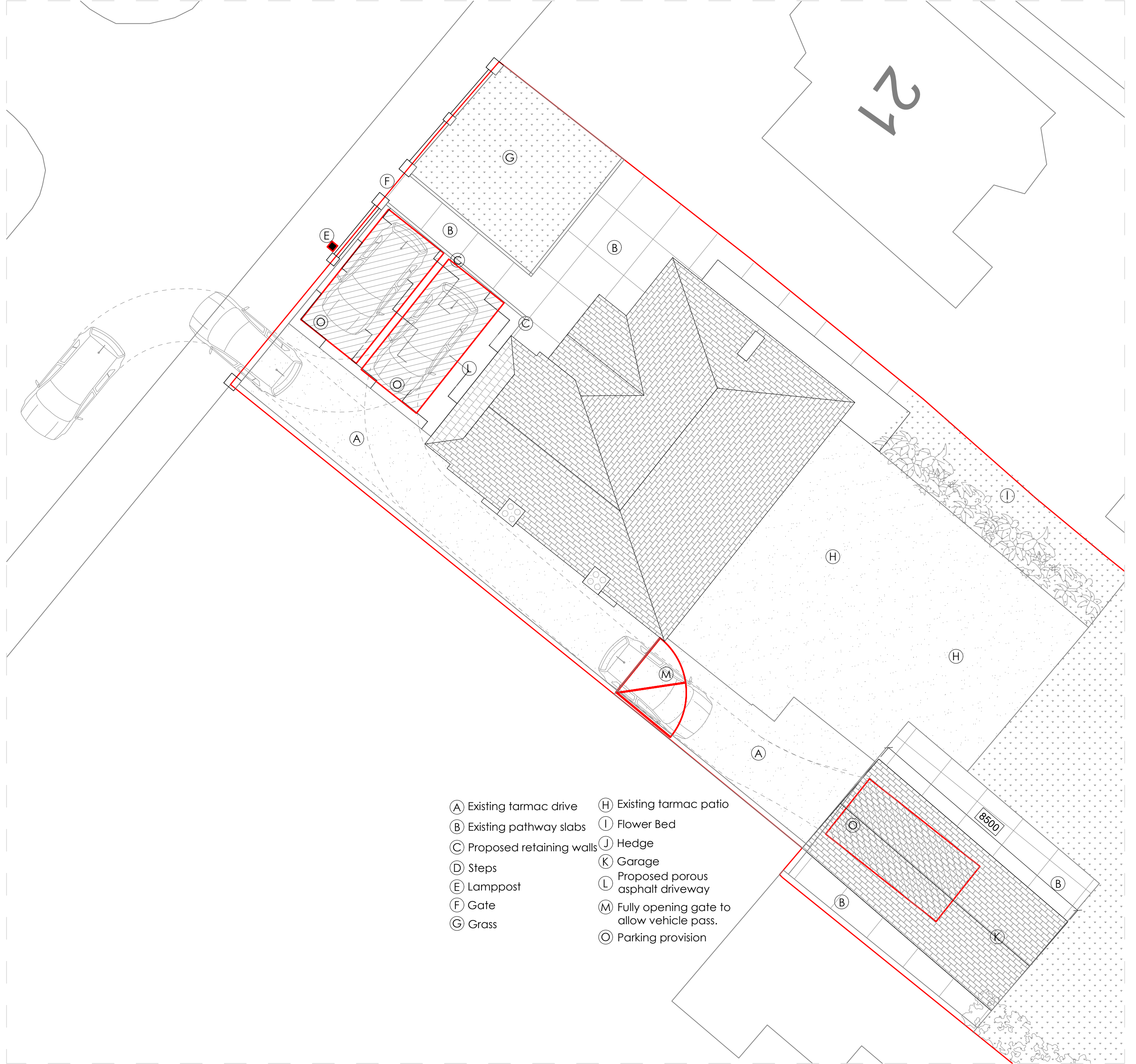
PP700 Auto Track - garage exit 1:100 @ A1
