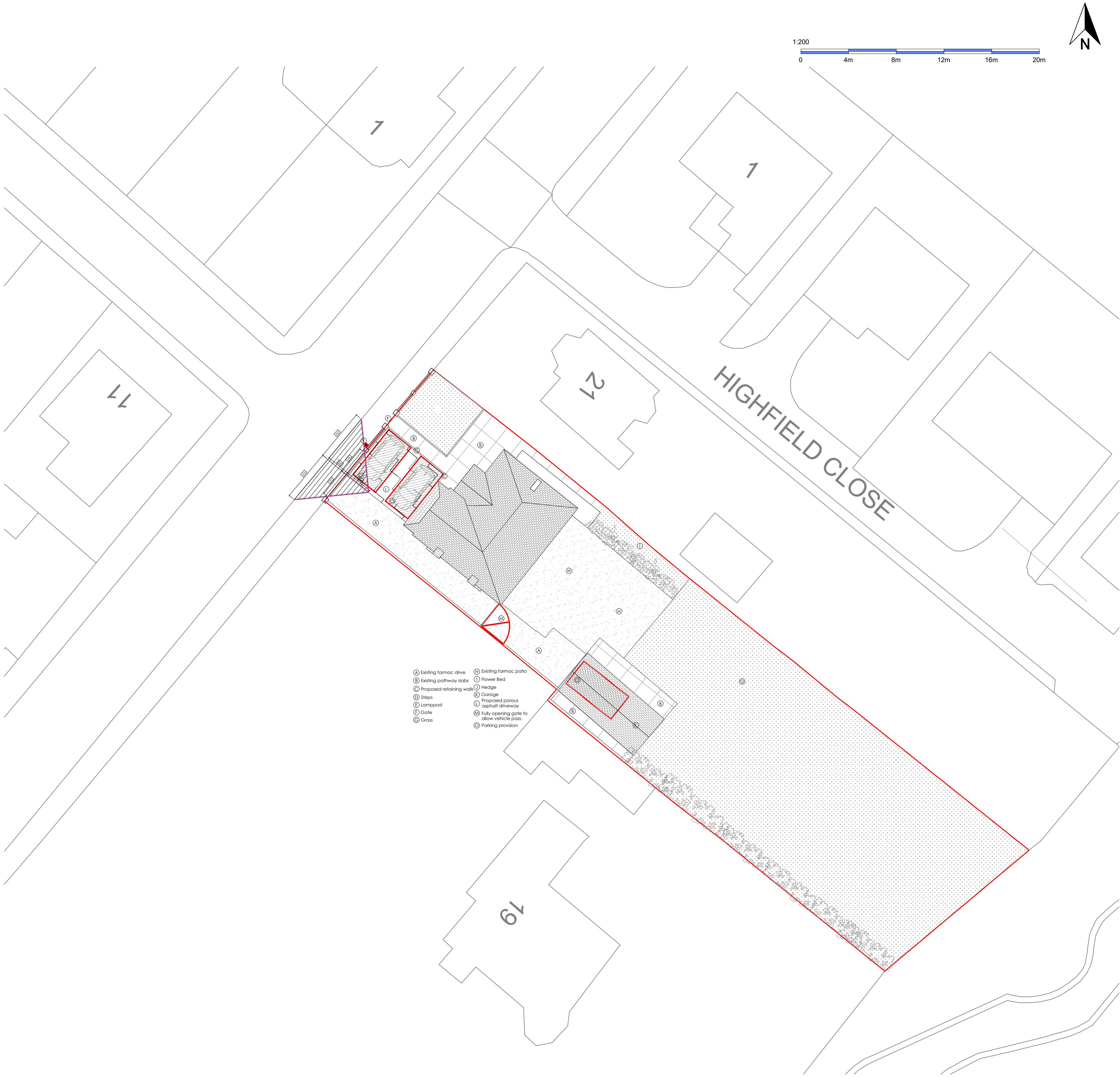
PP500 Pedestrian visibility splay 1:200 @ A1
