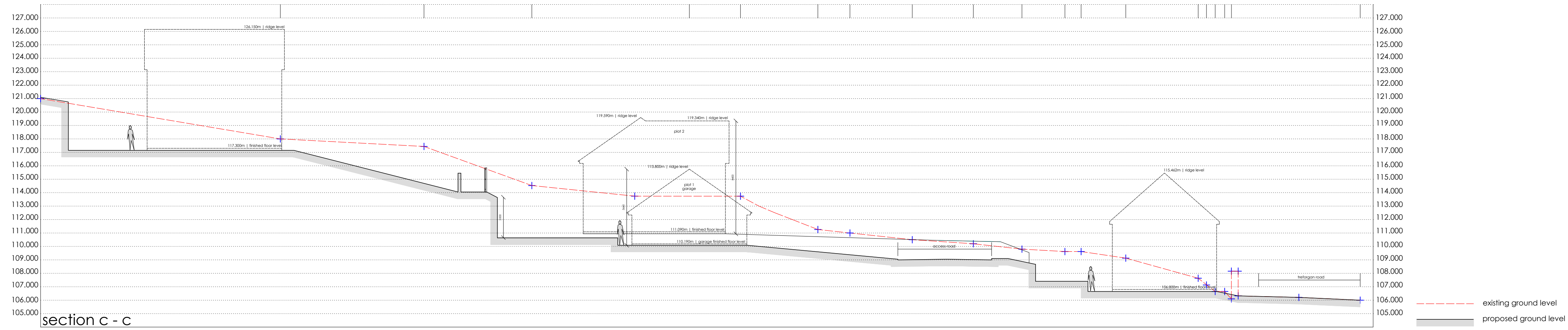
section b - b
