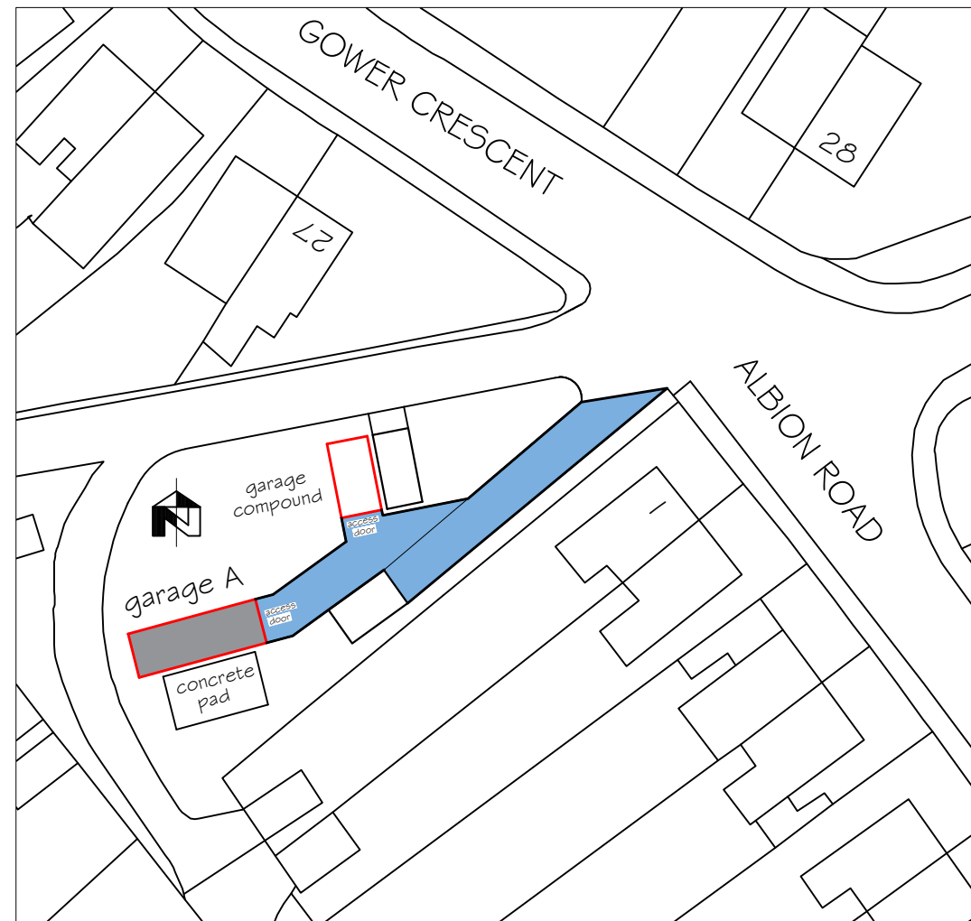
BLOCK PLAN 1:500
