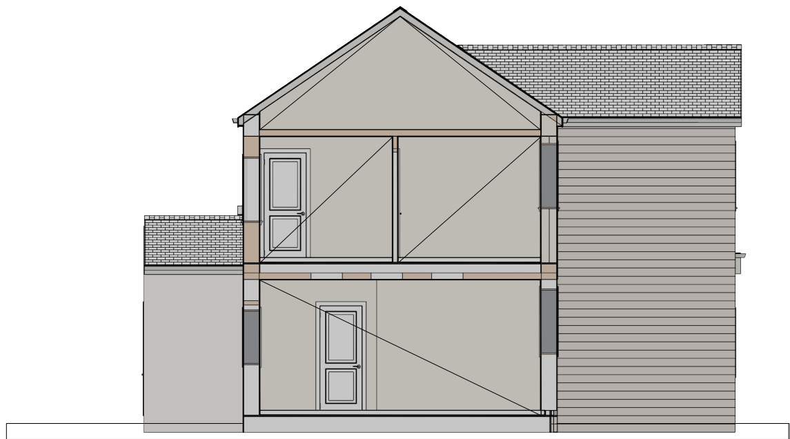
SECOND SIDE ELEVATION (SECTION THROUGH) PROPOSED
