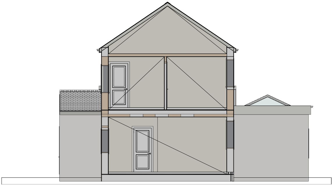
SECOND SIDE ELEVATION (SECTION THROUGH) EXISTING
