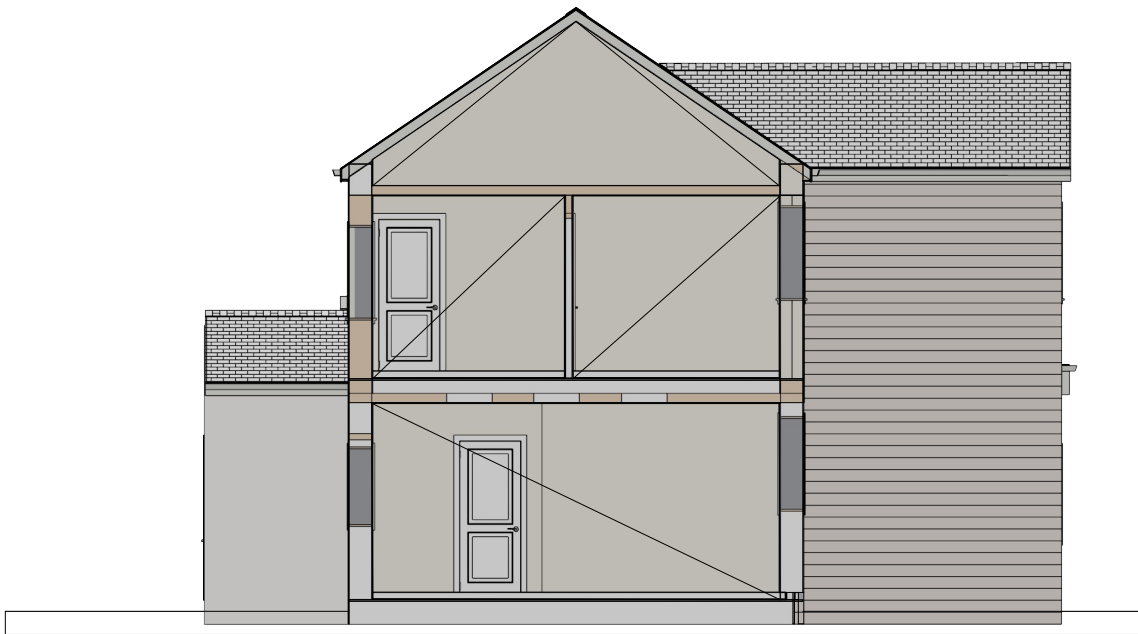
SEOCND SIDE ELEVATION (SECTION THROUGH) PROPOSED
