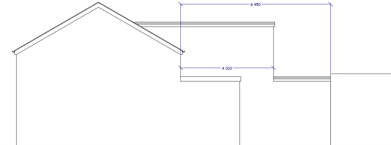
PROPOSED SECOND SIDE ELEVATION 1:100
