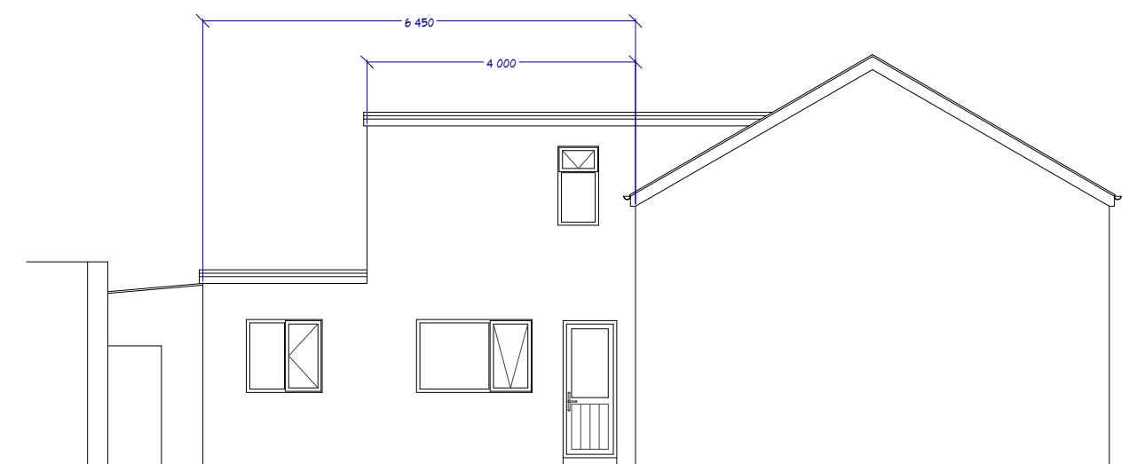
SIDE ELEVATION PROPOSED
