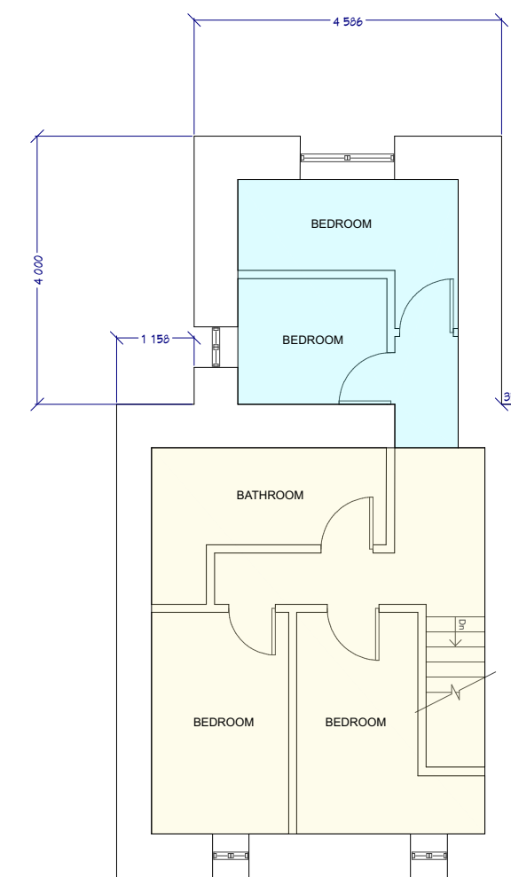
FLOOR PLANS PROPOSED
