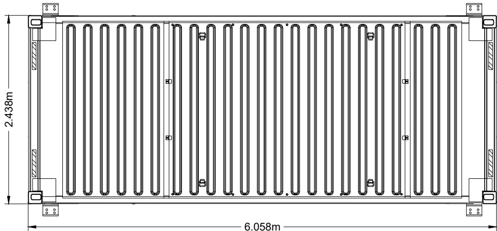
ROOF PLAN
