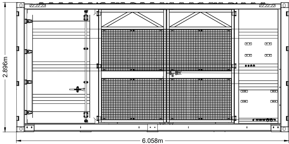
WESTERN ELEVATION
