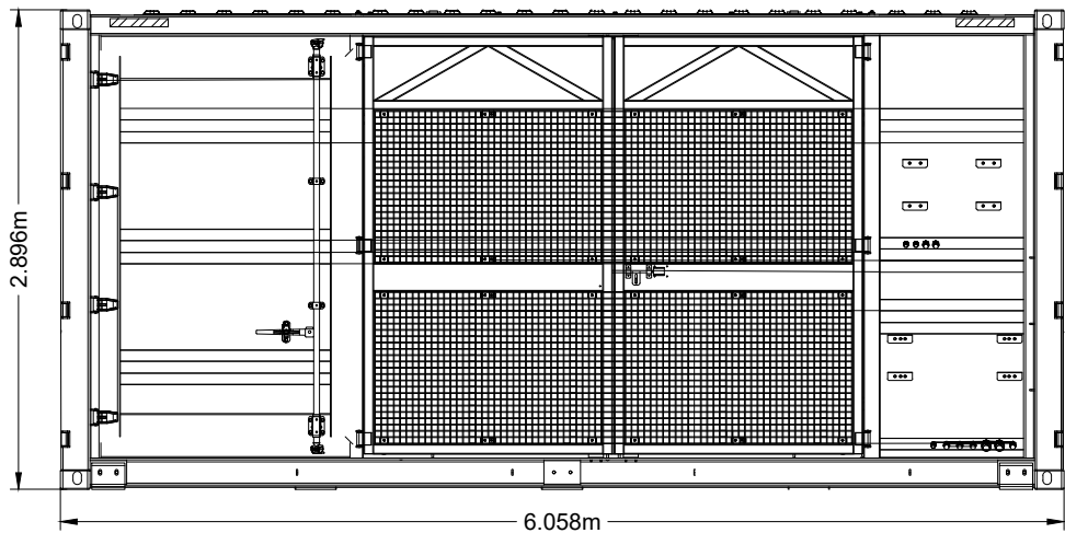
EASTERN ELEVATION
