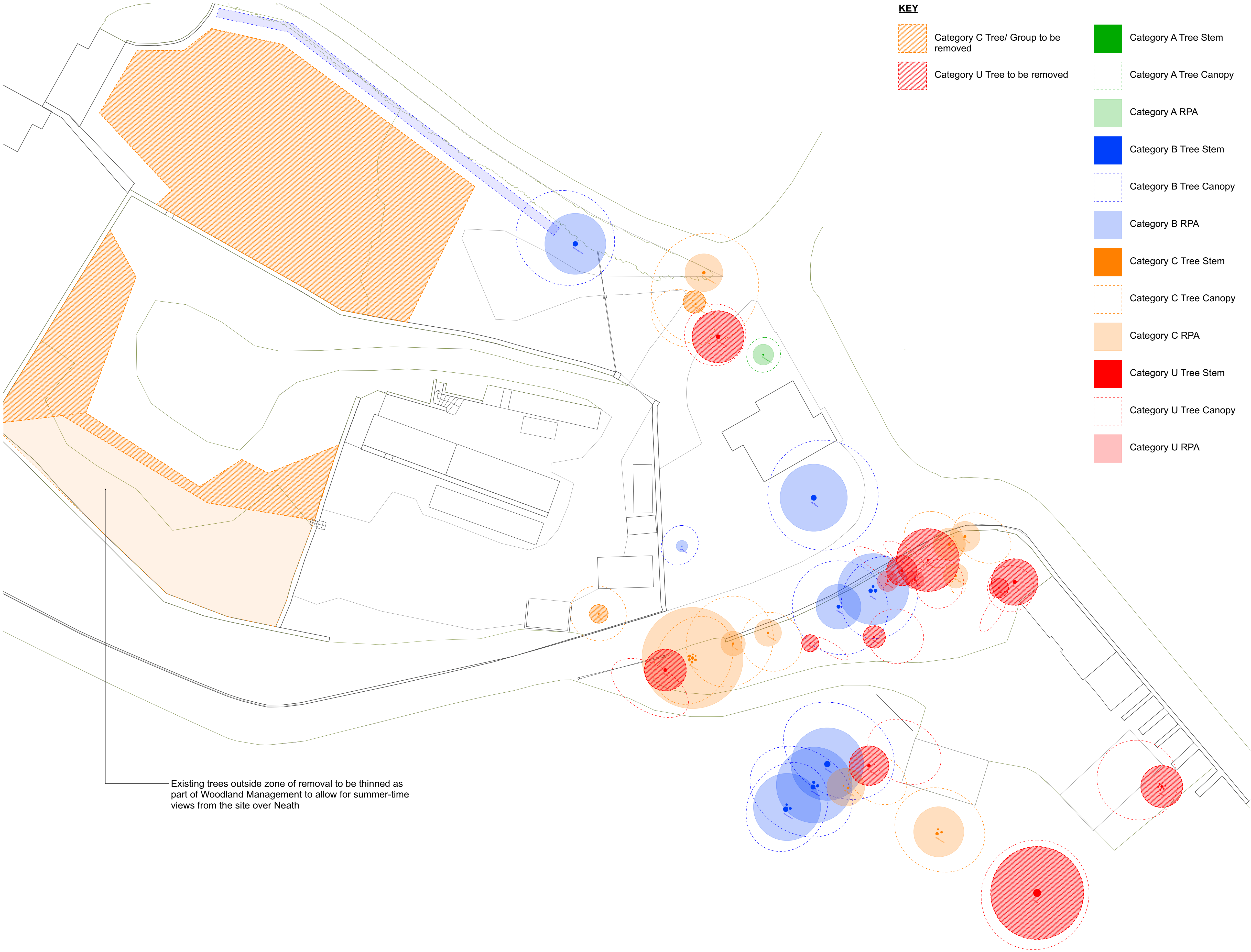
EX 00024.01 TREE REMOVAL PLAN: KITCHEN GARDEN + SERVICE YARD SCALE 1:250 @ A1, 1:500 @ A3
