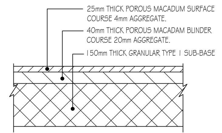
SECTION THRO' PROPOSED DRIVEWAY
