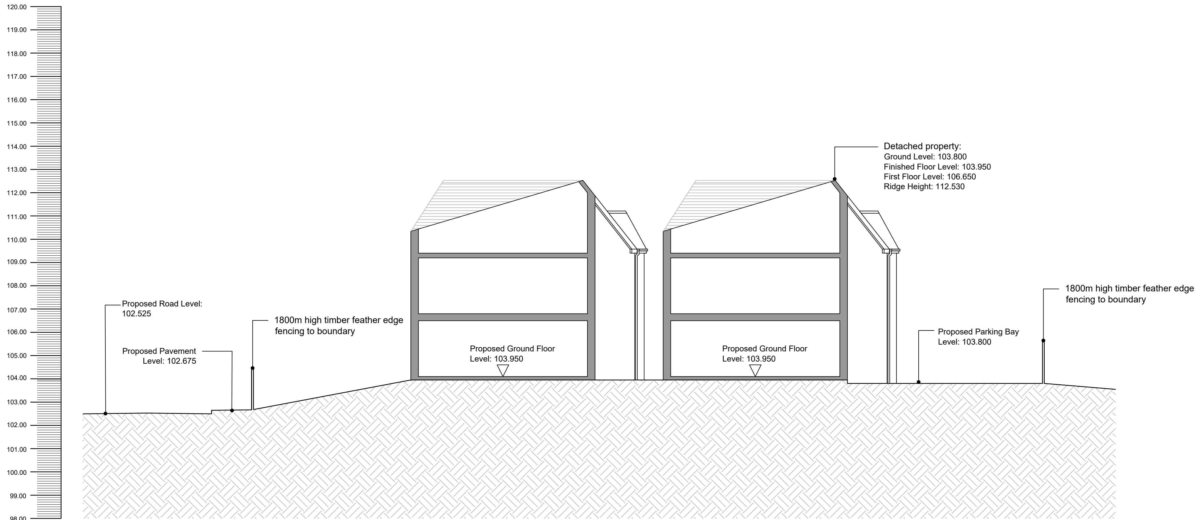
PROPOSED SECTION C-C SCALE 1:100 @ A1
