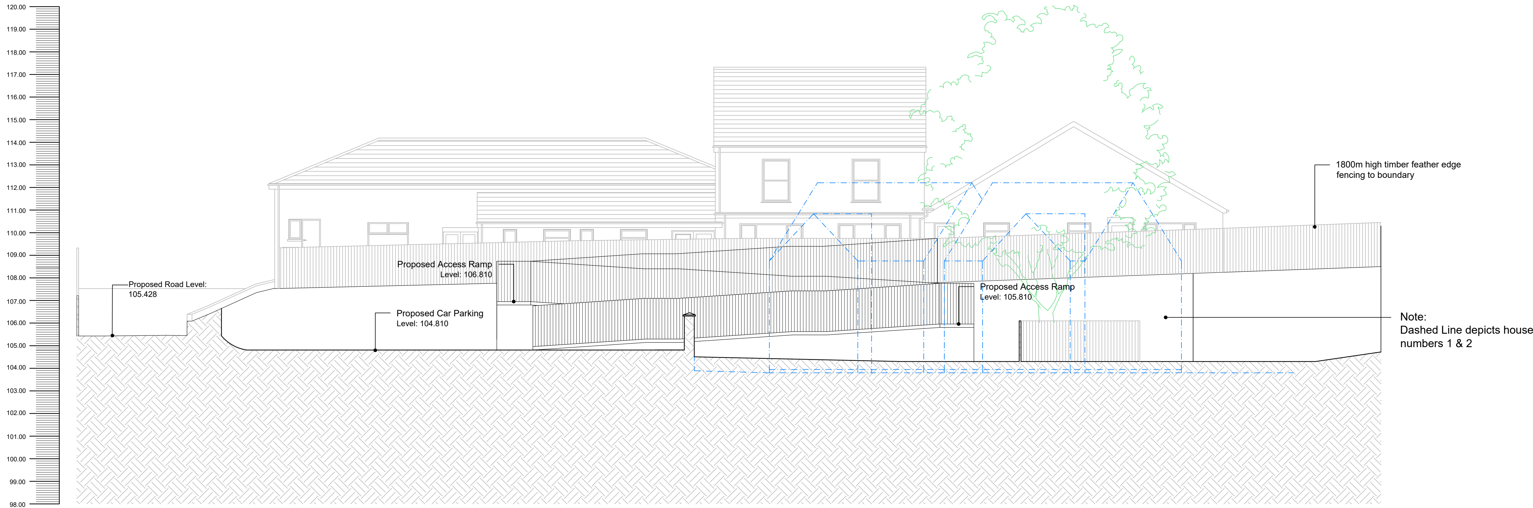
PROPOSED SECTION D-D SCALE 1:100 @ A1
