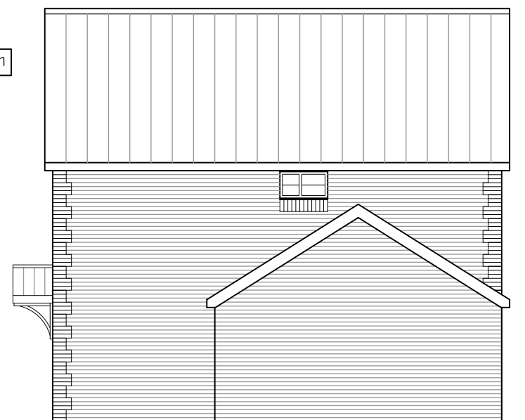
PROPOSED SIDE ELEVATION (North)
