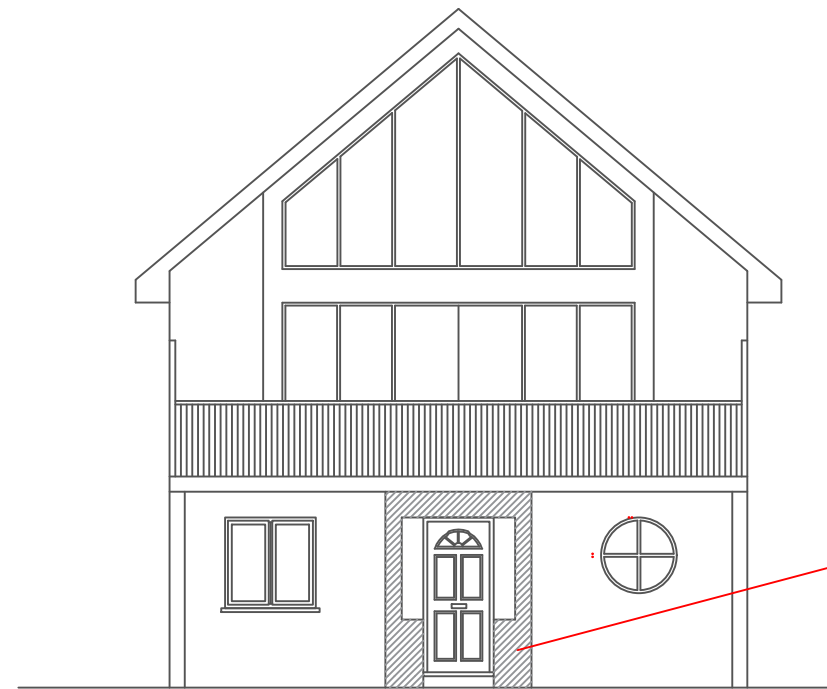
Front (South West) Elevation
