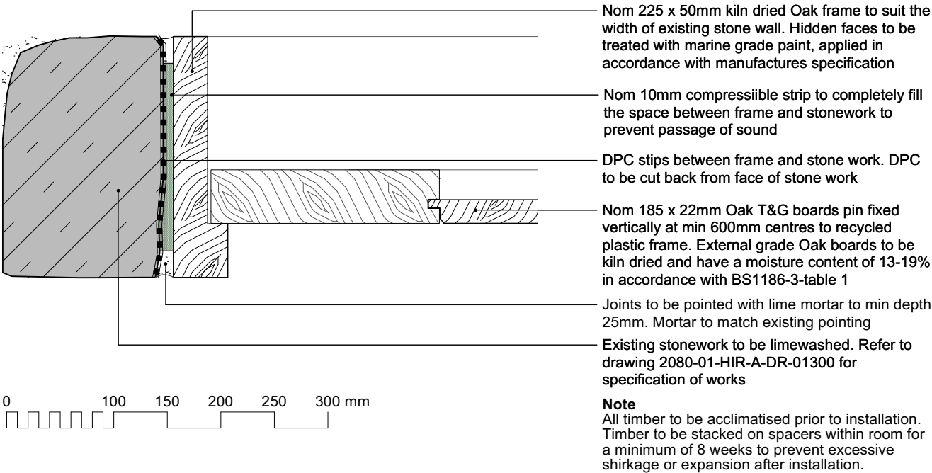
P 03782.4 JAMB DETAIL SCALE 1:5 @ A3
