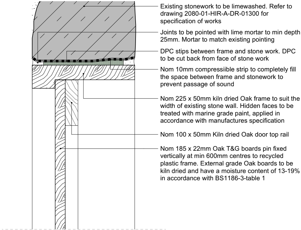
P 03782.5 DOOR SECTION HEAD DETAIL SCALE 1:5 @ A3
