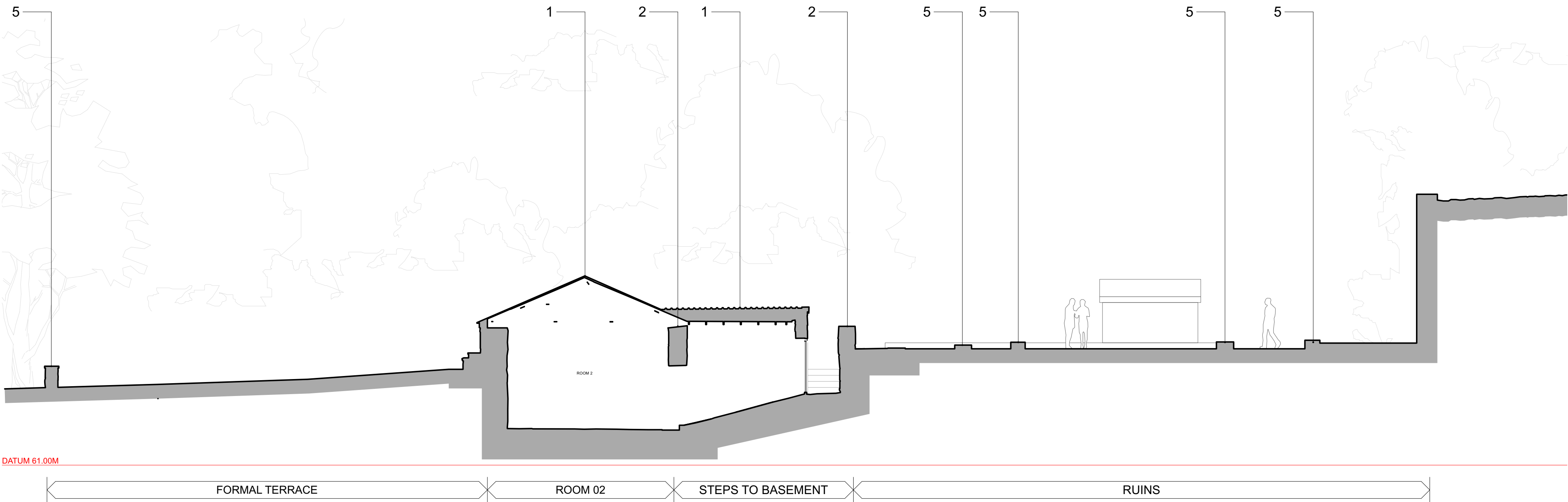
EX 03051.02 SECTION DD SCALE 1:100 @ A1, 1:200 @ A3
