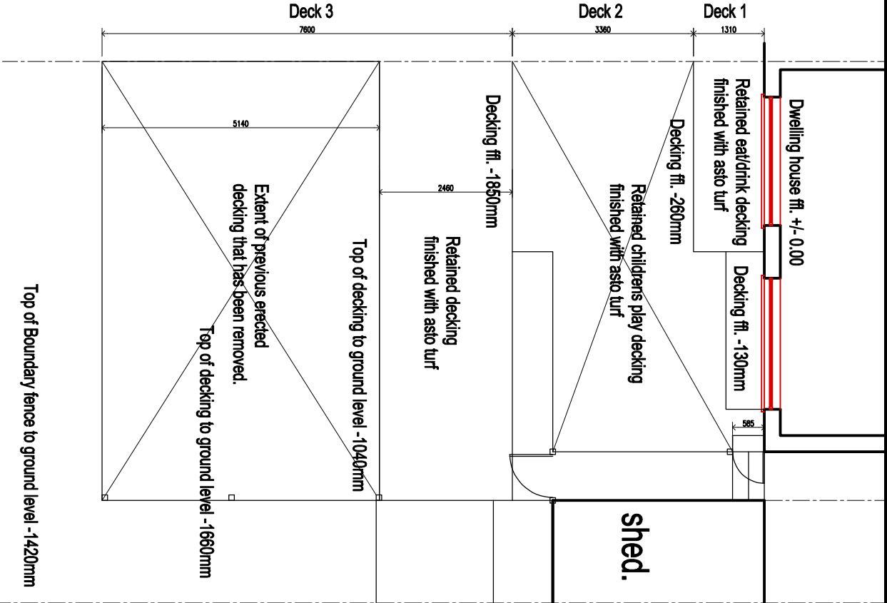
EXISTING REAR SITE PLAN.
