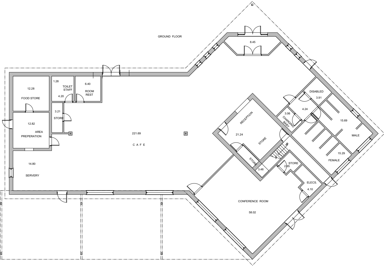
EX 020.1 GROUND FLOOR PLAN AS EXISTING SCALE 1:100 @ A1 / 1:200 @ A3
