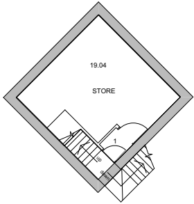
EX 020.2 FIRST FLOOR PLAN AS EXISTING SCALE 1:100 @ A1 / 1:200 @ A3
