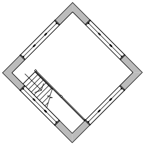
EX 020.3 SECOND FLOOR PLAN AS EXISTING SCALE 1:100 @ A1 / 1:200 @ A3
