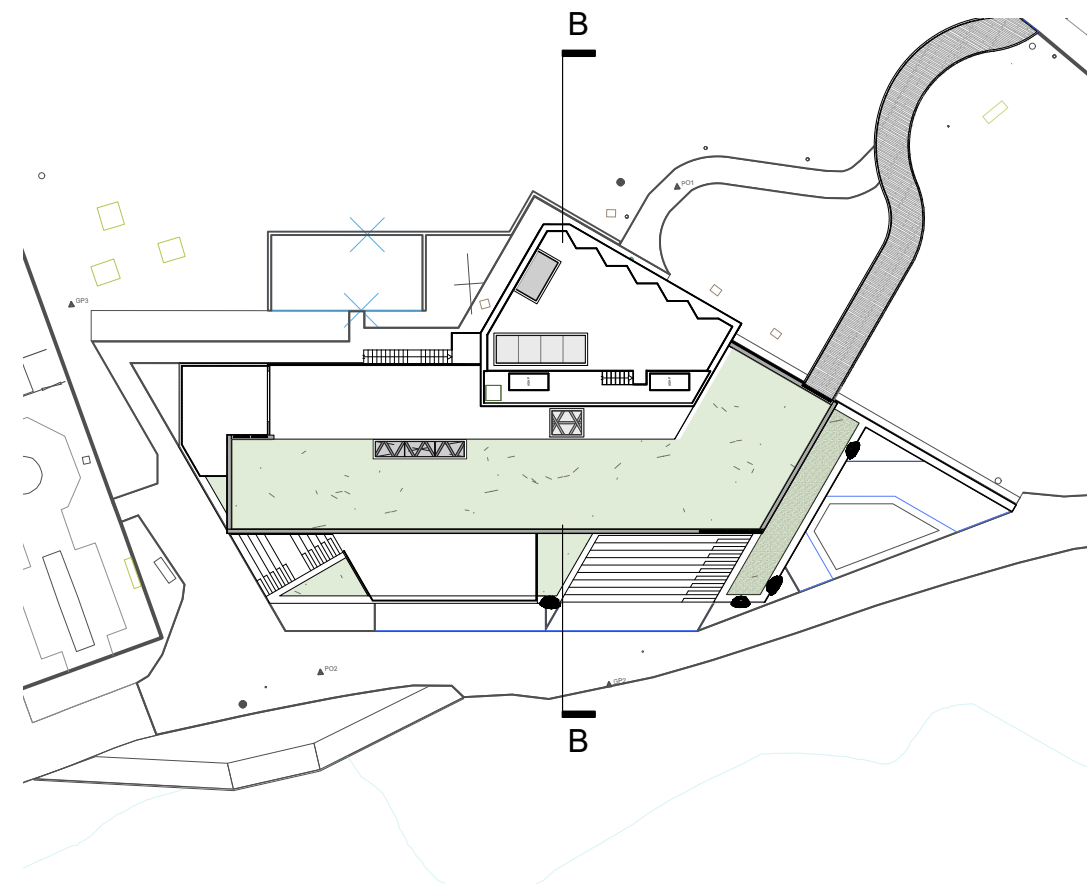
03510.2 KEY PLAN SCALE NTS
