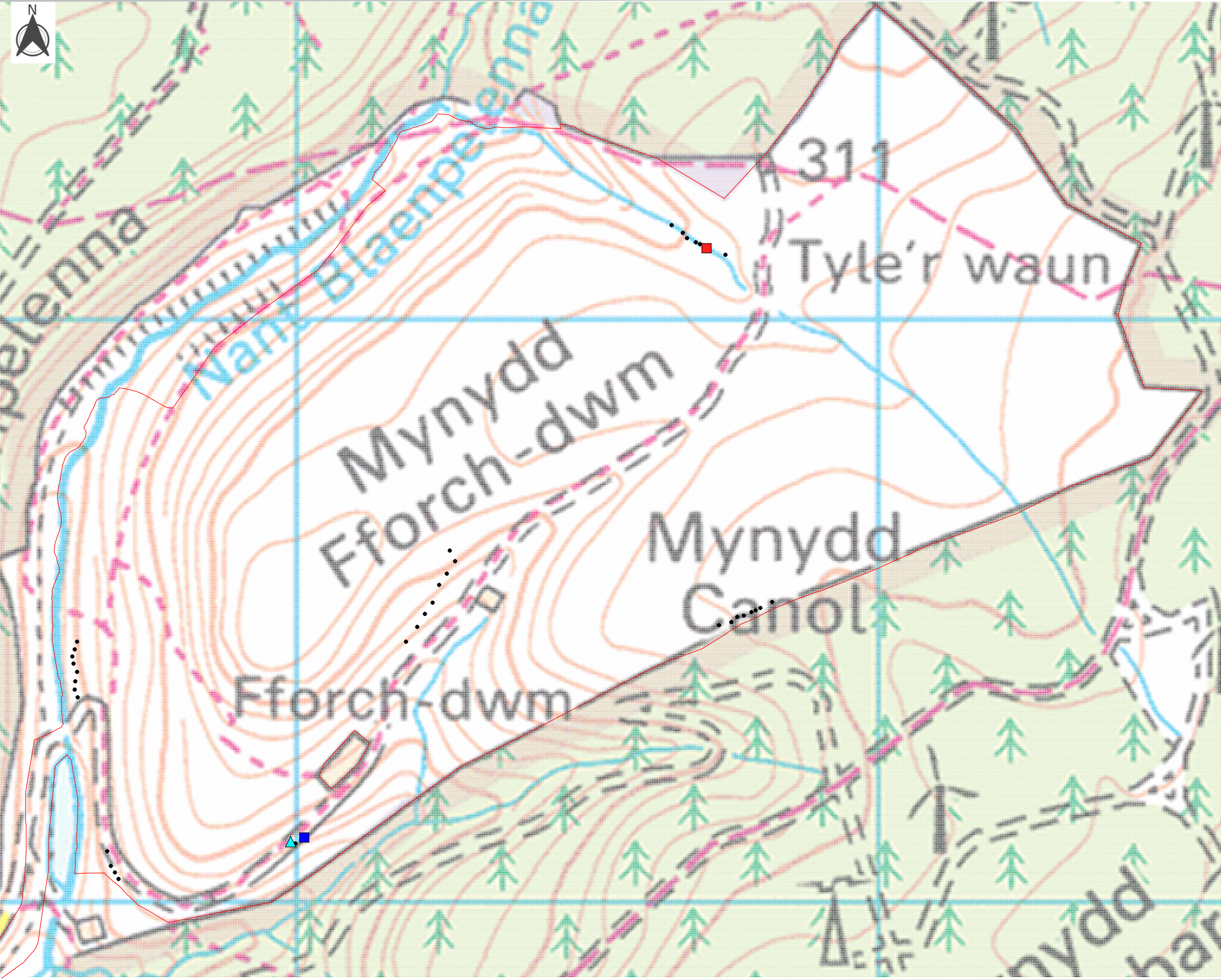
Figure 9.5b Reptile Survey
