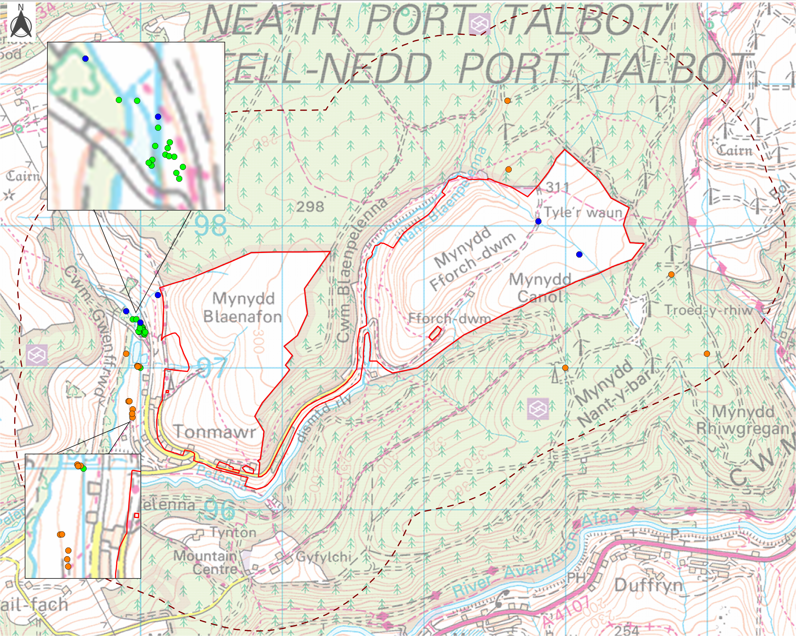
Figure 9.2b Existing Ecological Records (Reptiles)
