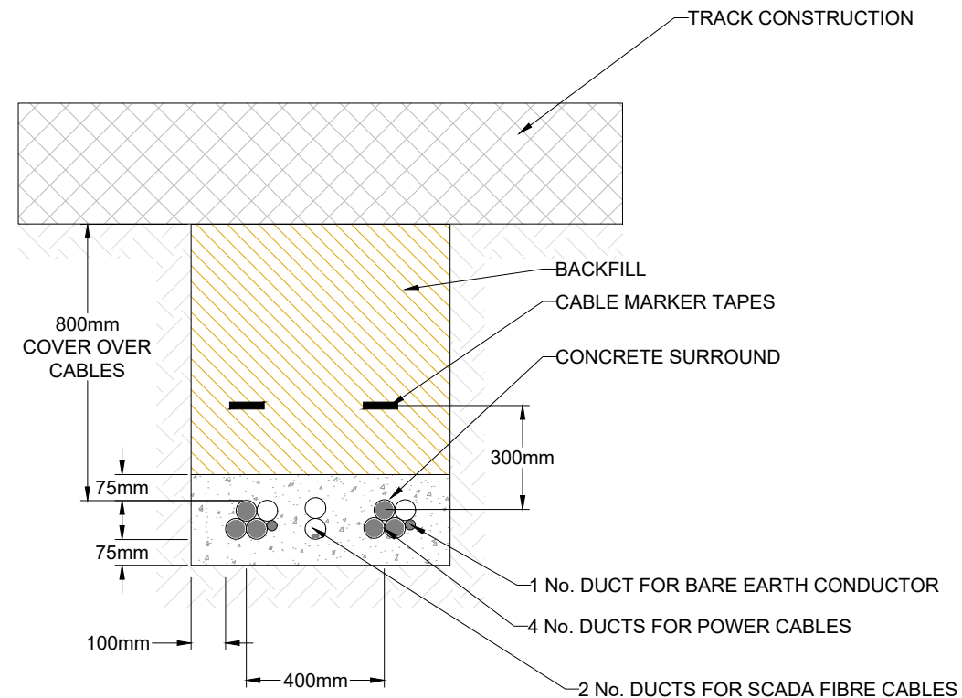
DOUBLE CIRCUIT
