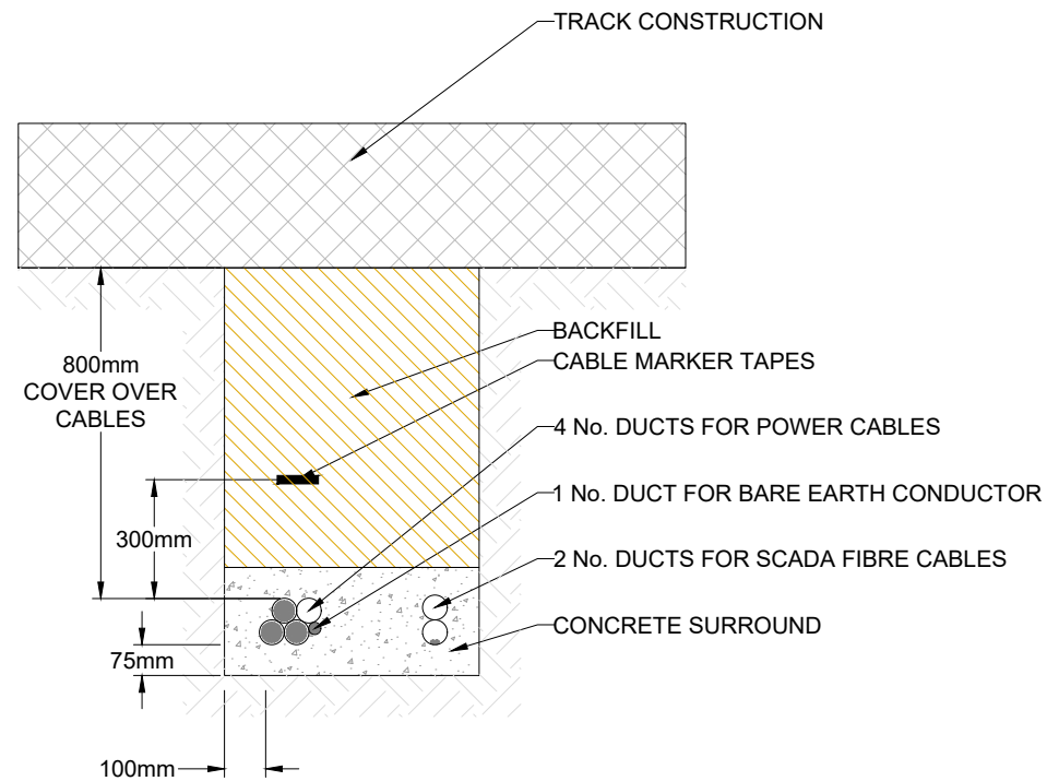
SINGLE CIRCUIT
