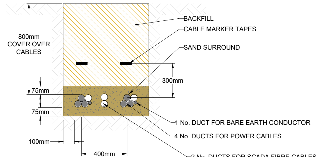
DOUBLE CIRCUIT
