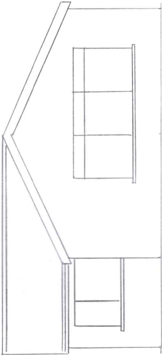
FRONT ELEVATION PROPOSED
