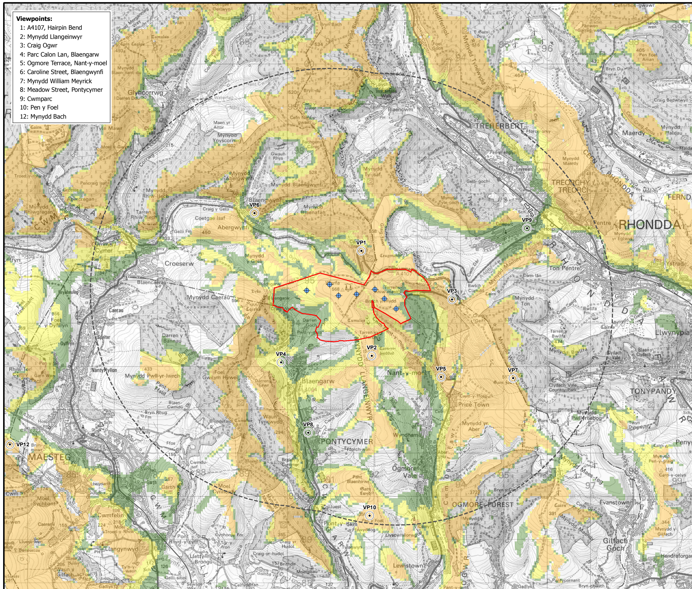
FIGURE 1 Zone of Theoretical Visibility to Turbine Tip Height
