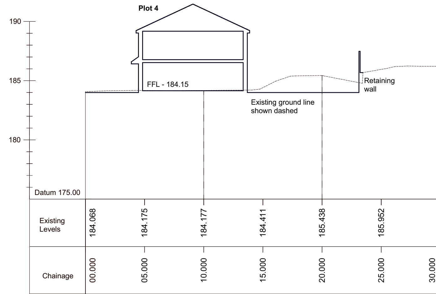
Section C-C
