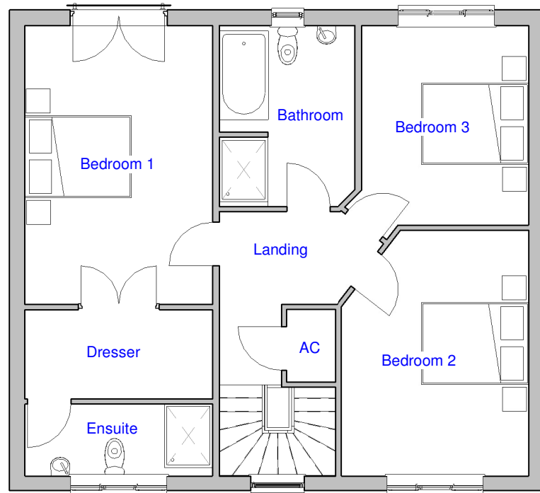
House 2 - First Floor
