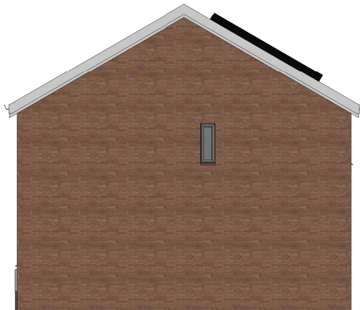
House 1 - Side Elevation 1
