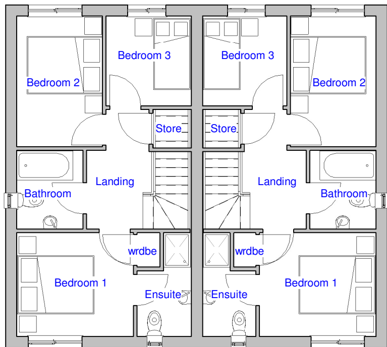
House 1 - First Floor
