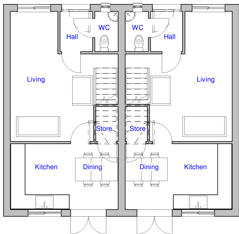
House 1 - Ground Floor
