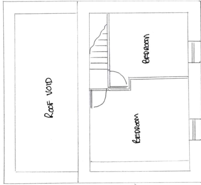
First floor PLAN EXISTING
