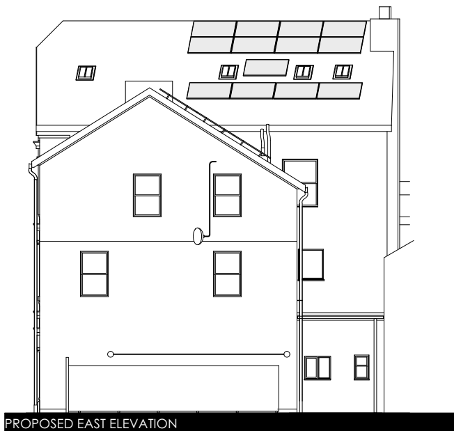
PROPOSED EAST ELEVATION
