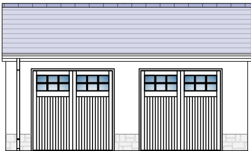
Garage Front Elevation.
