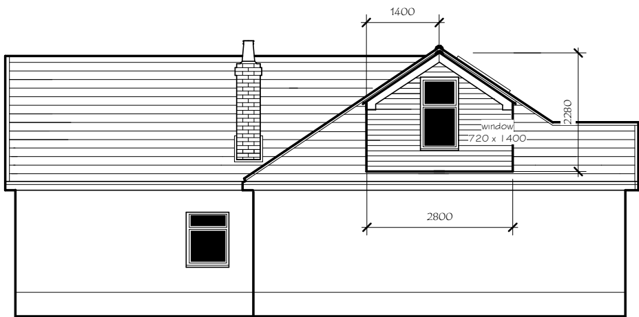
SIDE ELEVATION Facing North
