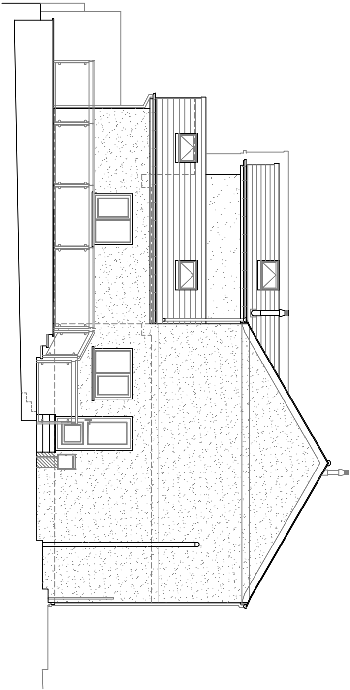
PROPOSED LH SIDE ELEVATION
