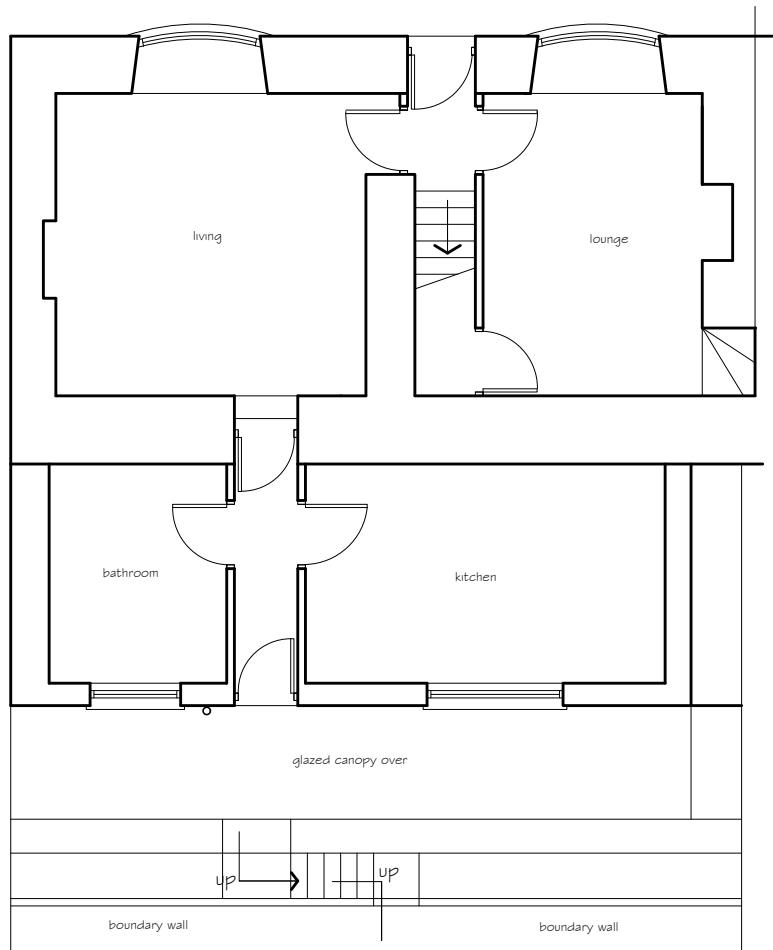
Proposed Ground Floor Plan - NO CHANGES
