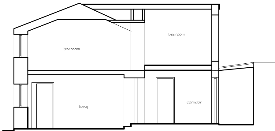
Proposed X Section
