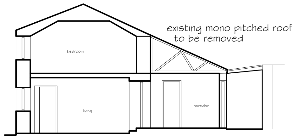
Existing X Section
