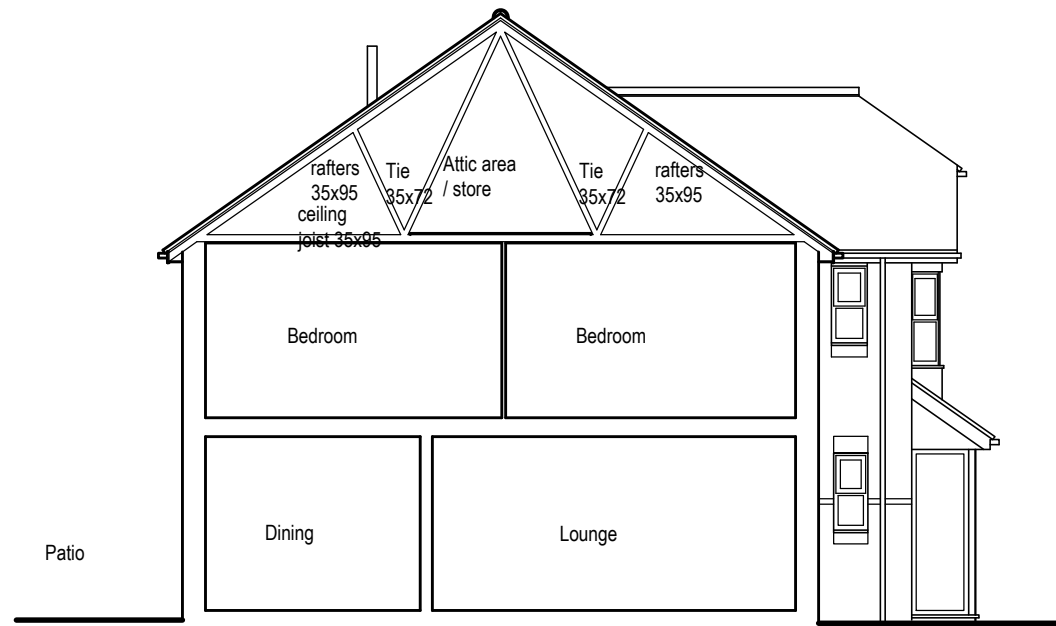
Existing Section AA
