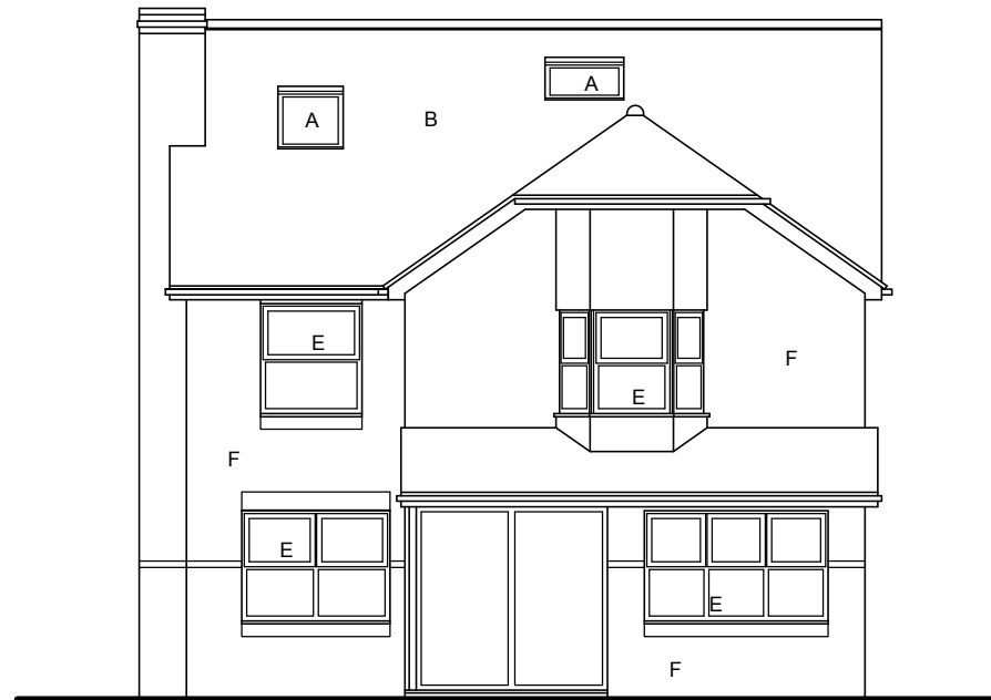
Front elevation (South East)
