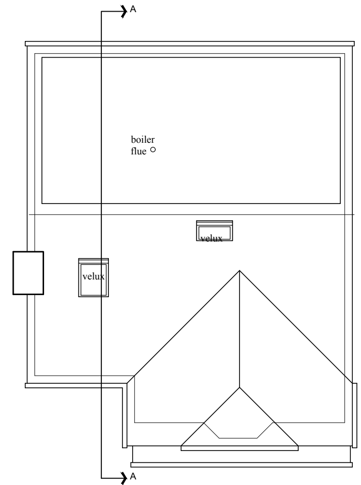
Proposed Roof floor plan
