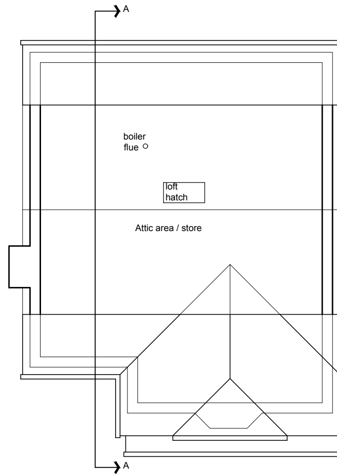
Existing Attic floor plan
