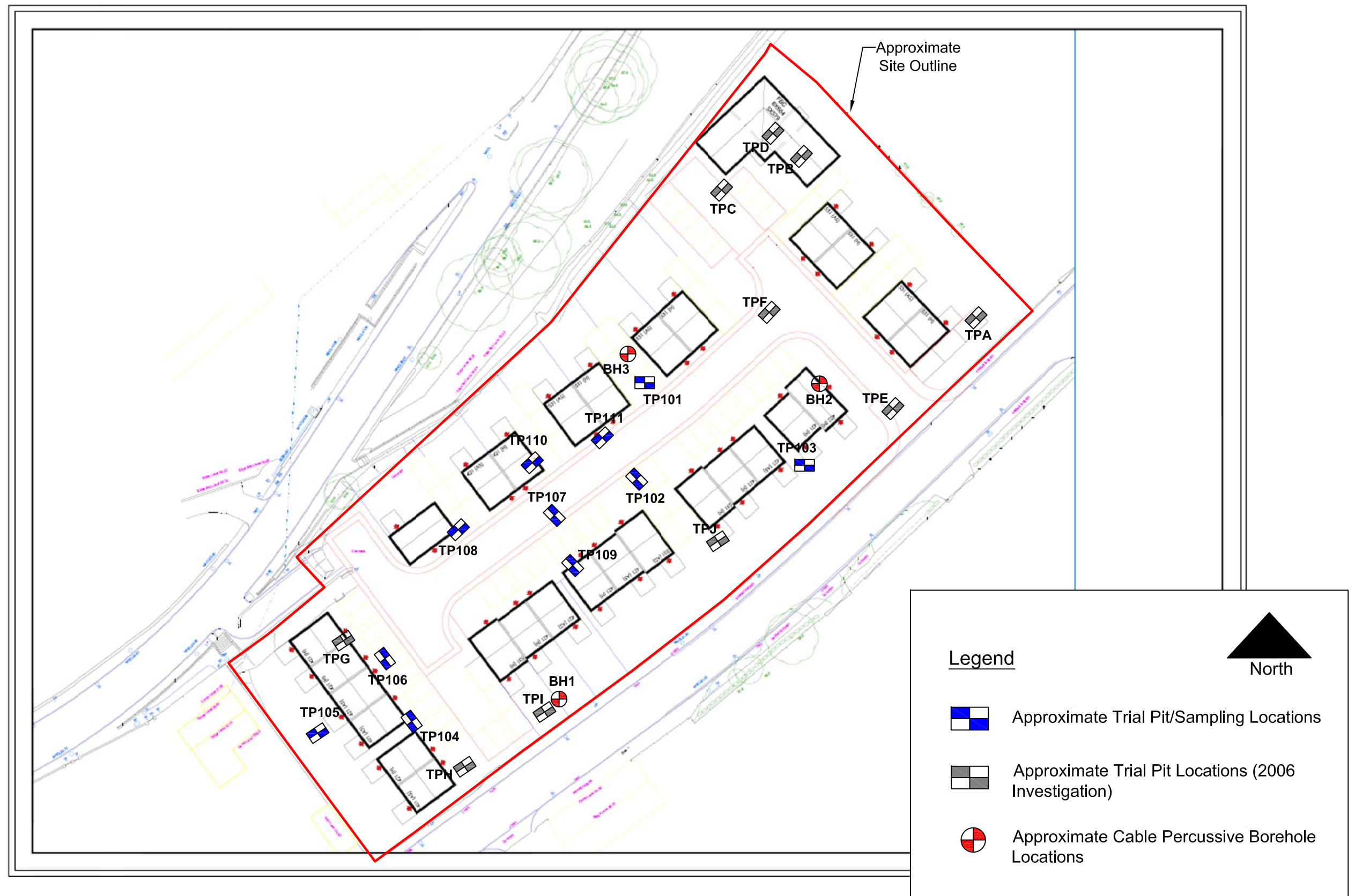
Figure 3: Site Plan (Proposed Layout)
