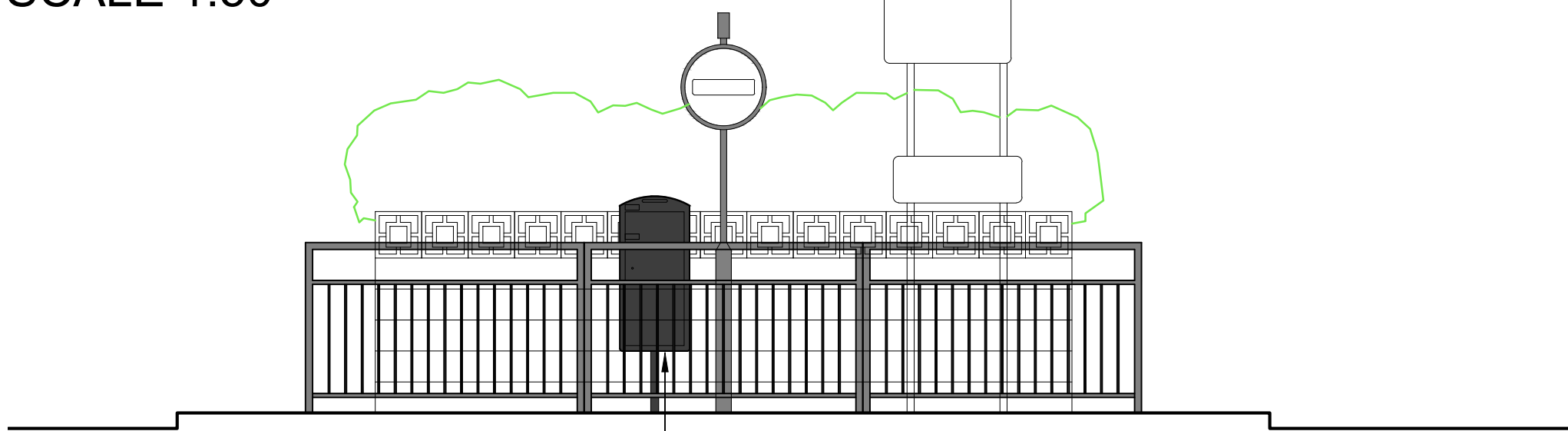
PROPOSED ELEVATION FROM JUNCTION SCALE 1:50
