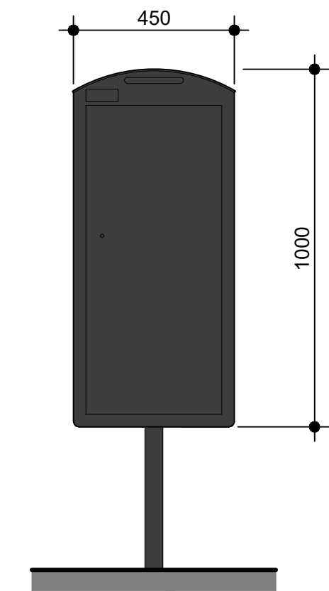
PROPOSED DOUBLE POUCH BOX PLAN AND ELEVATION SCALE 1:20
